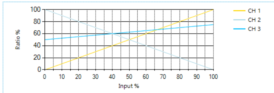
Figure 15. Example of INT Calibration Graph
