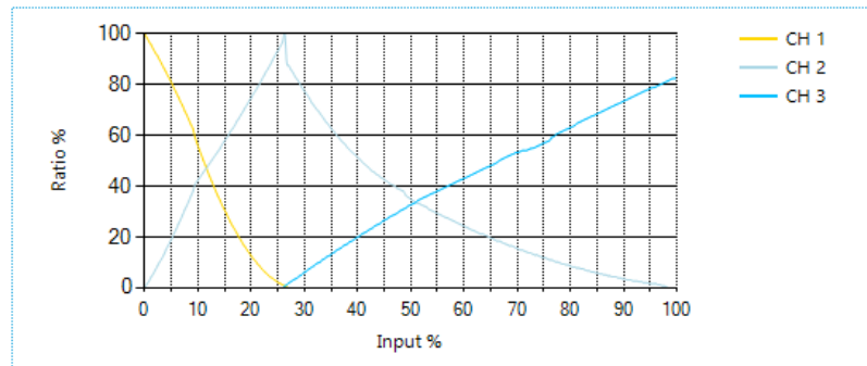
Figure 13: Example of CCT Calibration Graph
