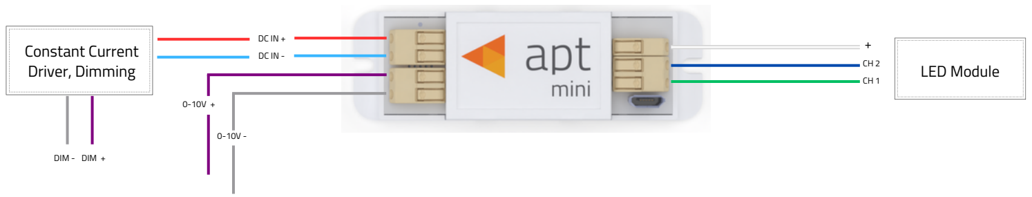
Figure 1 – APT-CC-VS-M1-xxxxTW Wiring Diagram
