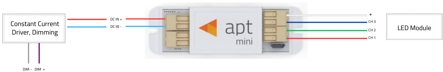
Figure 5 – APT-CC3-VS-M1-xxxxDW Wiring Diagram
