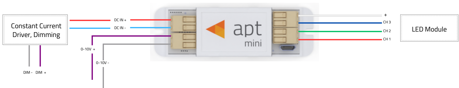
Figure 3 – APT-CC3-VS-M1-xxxxTW Wiring Diagram
