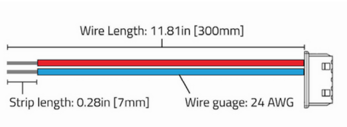
Figure 2 – Programmable Selectable White Cable Assembly
