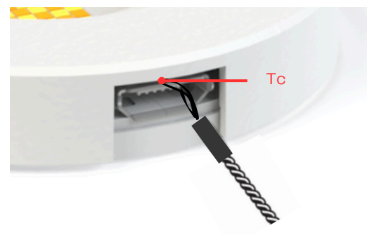
Figure 1 - Tc is measured on the metal sleeve of the micro-USB programming port. To measure Tc, insert thermal probe between micro-USB and top encasement of the ORB controller as shown.
