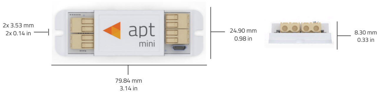
Figure 1 – Mechanical Drawing
