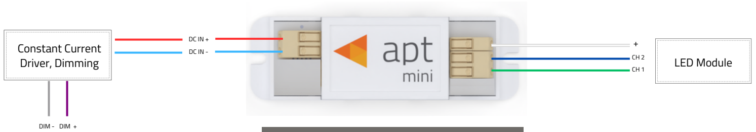
Figure 1 – APT-CC-VDW-M1-xxxx Wiring Diagram
