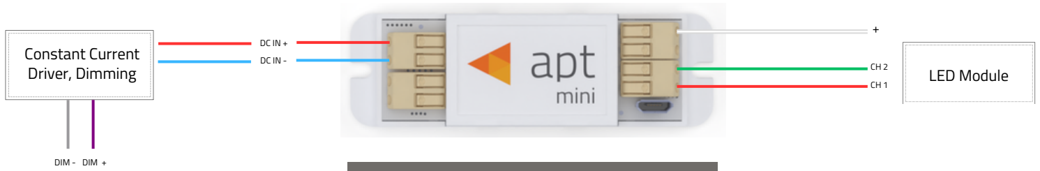
Figure 1 – APT-CC3-VS-M1-xxxxDW2 Wiring Diagram
