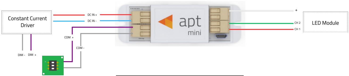
Figure 1– APT-CC3-VS-M1 -xxxxSW2 Wiring Diagram
