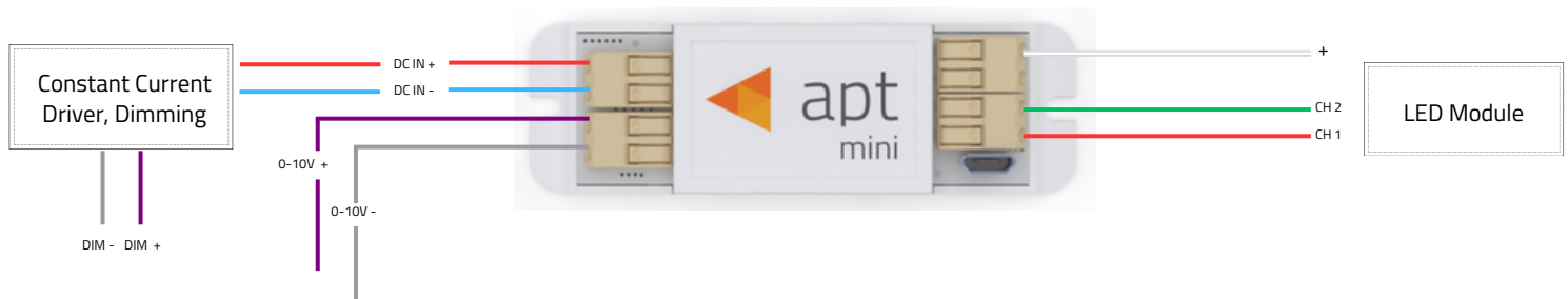
Figure 1 – APT-CC3-VS-M1-xxxxTW2 Wiring Diagram
