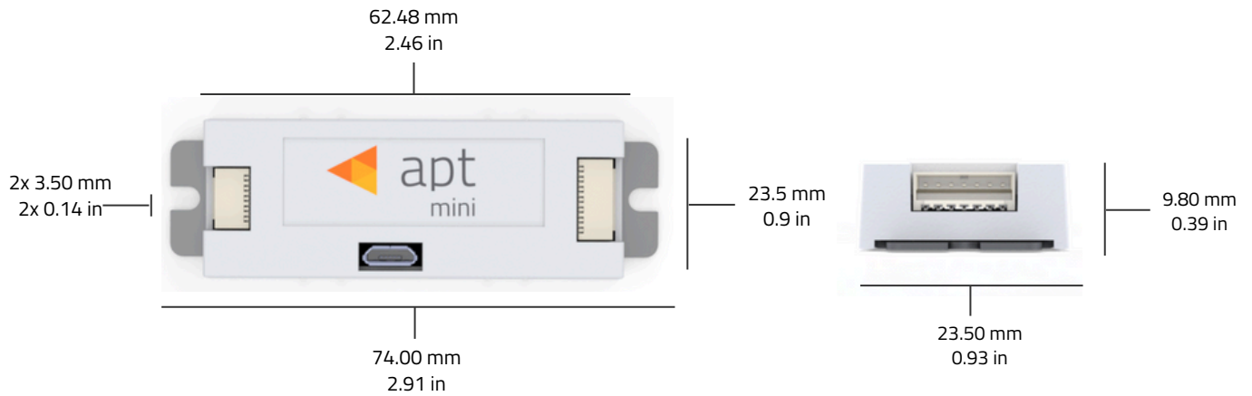
Figure 1 – Mechanical Drawing
